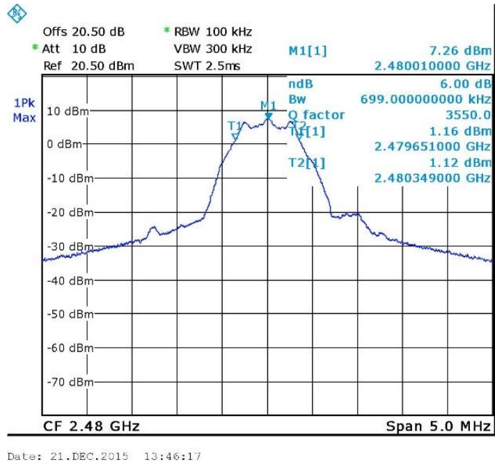
Figure 18. 2480.0 MHz
