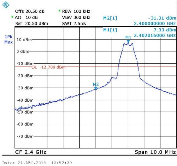
Figure 26 —Lower Band Edge
